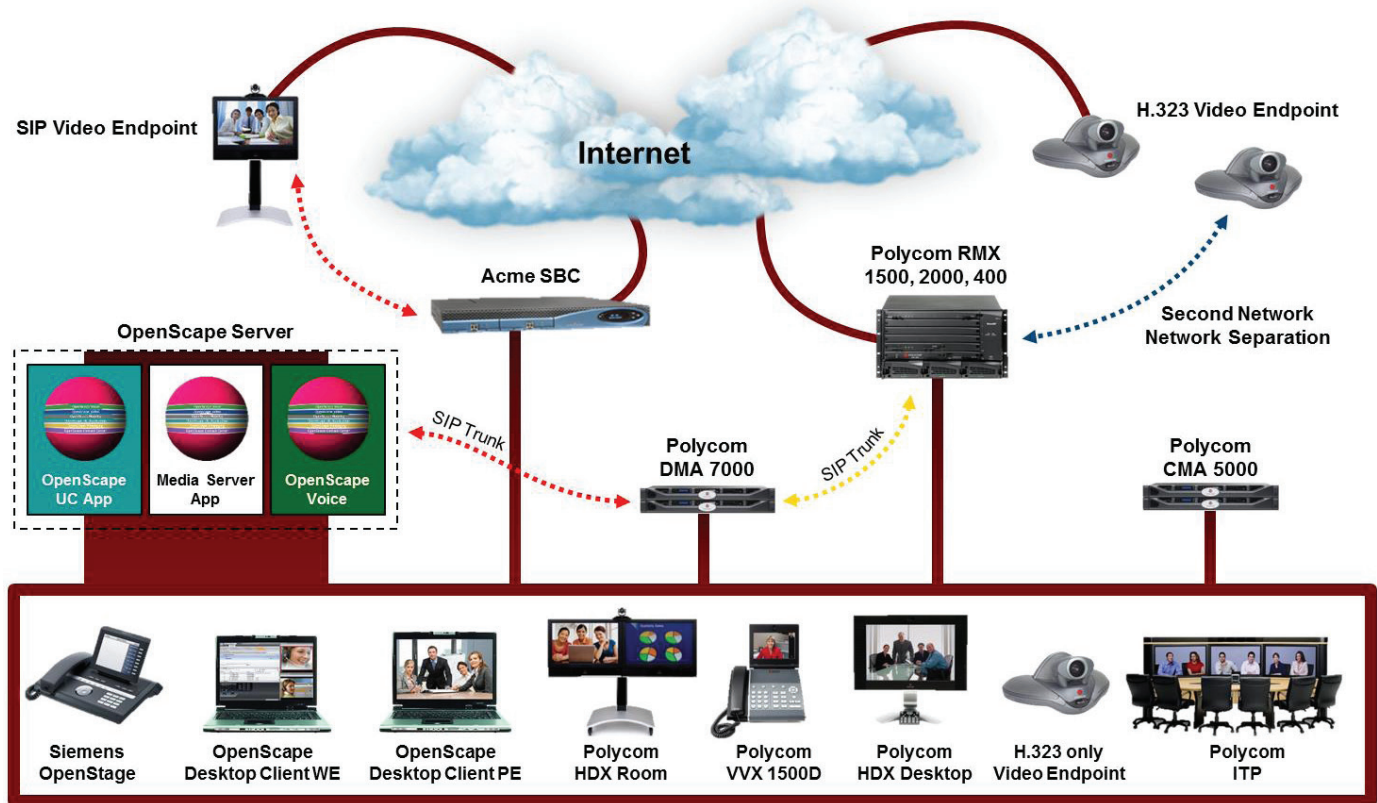
Figure 1: Solution Architecture for OpenScape Integration: HD video conferencing with voice, video and OpenScape Desktop Client video participants.
